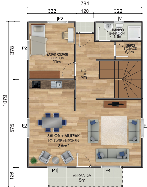
Zemin Kat Planı / Ground Floor Plan 73 m 2 + 6 m 2 = 79 m 2
